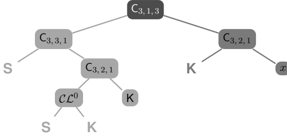
Figure 3: Colored tree representation of a combinator from the set \mathcal{C}_{3,1,3} .
