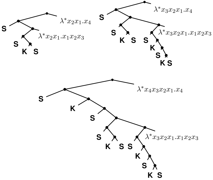
Figure 6: Three consecutive steps of the translation of the term \lambda x_4 x_3 x_2 x_1 . x_1 x_2 x_3 x_4 .
