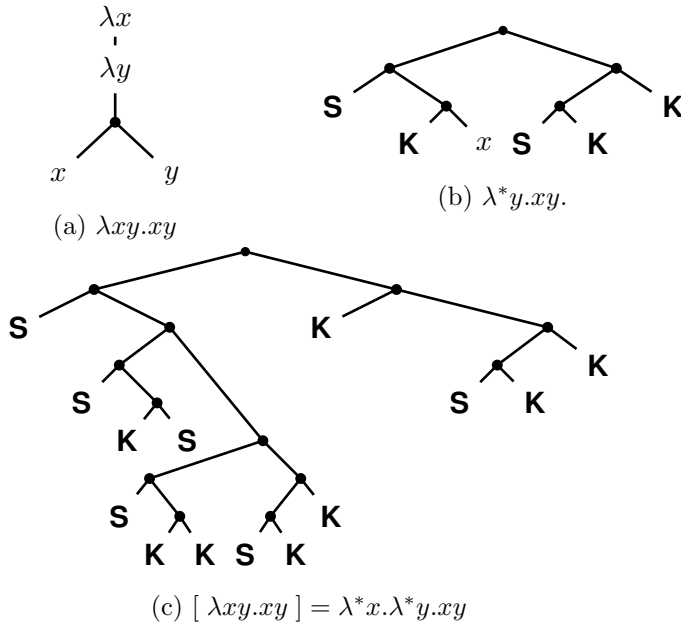
Figure 1: Visualization of some consecutive steps of the translation algorithm for the term \lambda xy.xy .
