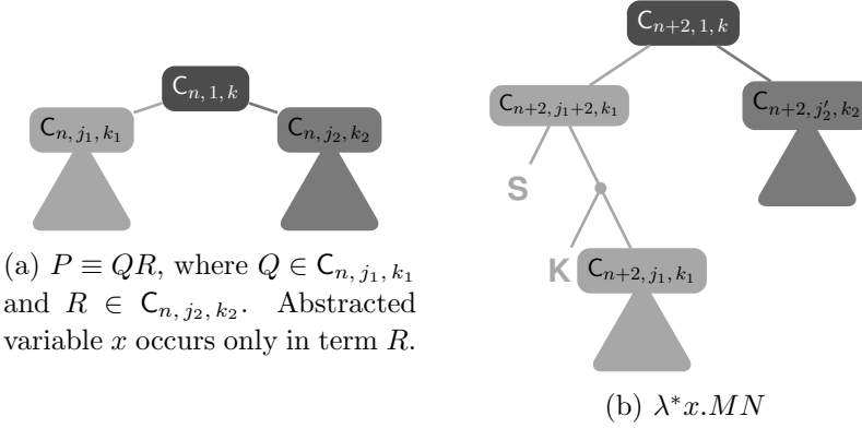
Figure 4: A term before and after applying the bracket abstraction.
