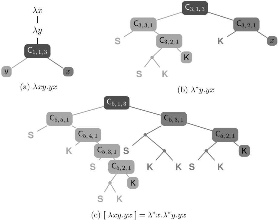
Figure 5: Step-by-step translation of the term \lambda xy.yx using the colored representation of terms of the set C_{n,j,k} .
